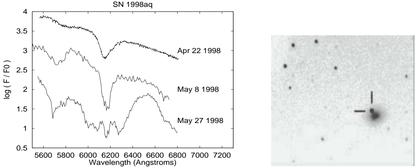
Fig. 1. Observed spectra of SN 1998aq (left panel) and CCD picture of NGC 3982 showing SN 1998aq (right panel). The epochs of spectroscopic observations are indicated on the right side of each spectrum.
